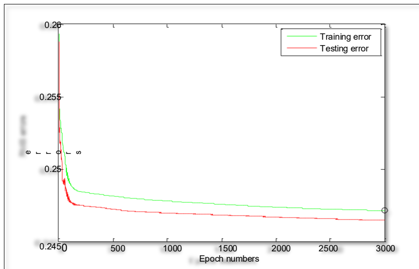
Figure 6: ANFIS performance
