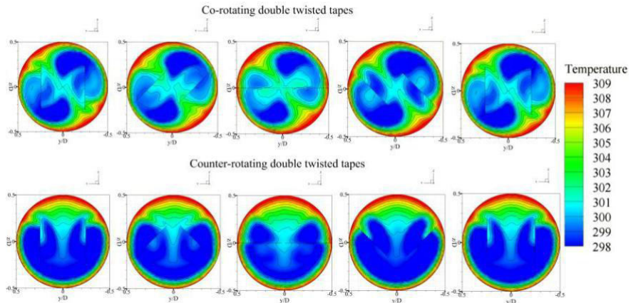
Figure 7: Details of temperature contours in transverse planes for double twisted tapes at Re = 800 and TR = 2 .
