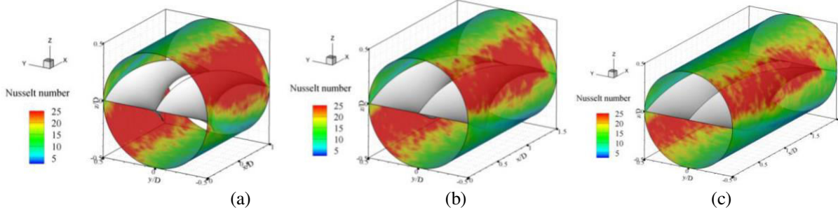
Figure 9: Nu_x Contours for (a) co-rotating case and (b) counter-rotating case of double twisted tapes at Re = 800 and TR = 2 .
