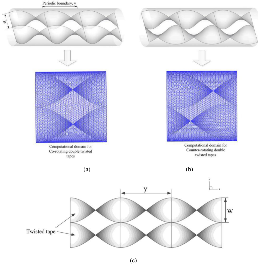
Figure 1: (a) tube geometry and computational domain for co-rotating case and (b) tube geometry and computational domain for counter-rotating case and (c) details of double twisted tapes.
