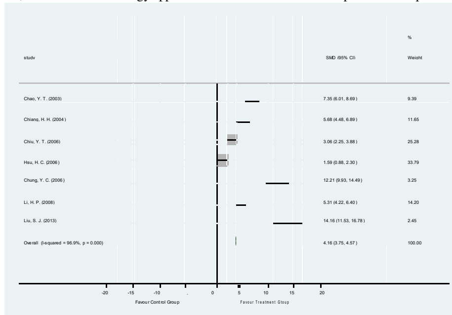
Figure 2: The Forest Plot of These 7 Theses in This Study of Patients' Knowledge with the Weights from Fixed Effects Analysis
