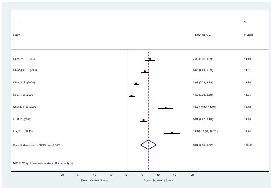
Figure 3: The Forest Plot of These 7 Theses in This Study of Patients' Knowledge with the Weights from Random Effects Analysis
