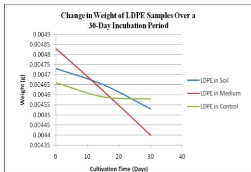
Figure 4: Average weight loss of LDPE plastics cultivated in soil and in SDA medium after 30 days.
